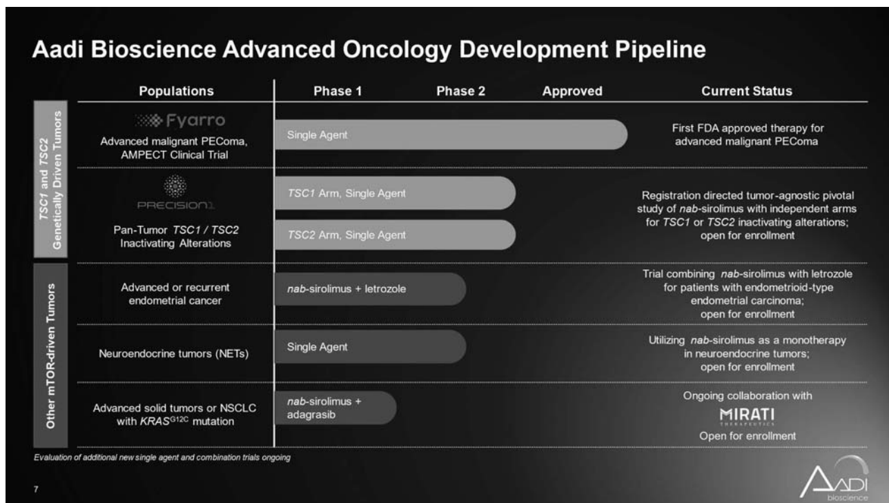
Figure 5 – Pipeline
